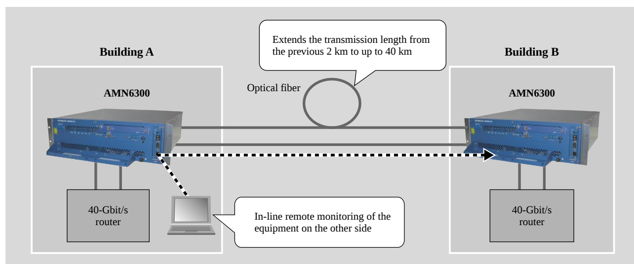
Fig. 1—Example of System Configuration Using AMN6300.
