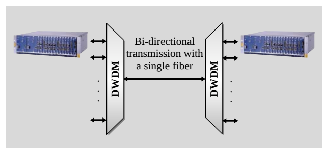
Fig. 5—32-wavelength Bi-directional Transmission with a Single Fiber DWDM System Using AMN6200 CWDM Platform. A CWDM-system platform is used, and a compact, easy-to-use, large-capacity DWDM system is provided.
