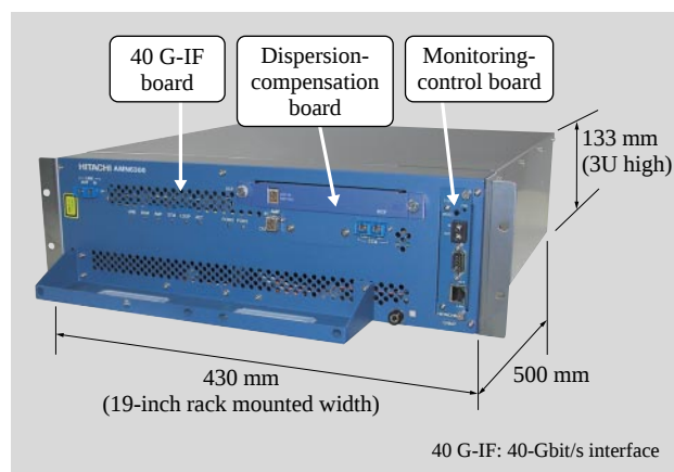
Fig. 3—External View of 40-Gbit/s Extender System “AMN6300.”
