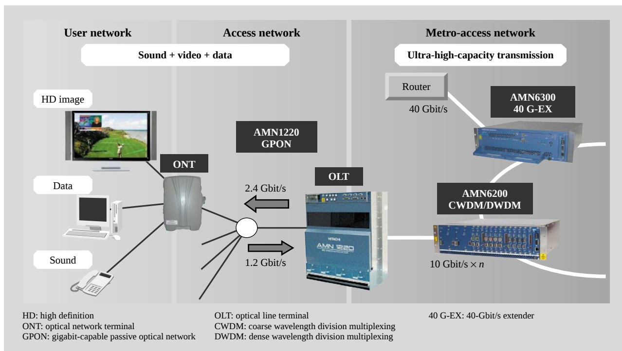
Fig. 1—GPON, 40 G-EX, Bi-directional Transmission with a Single Fiber DWDM System for Accomplishing Key Roles in the Era of Converged Broadcasting and Telecommunications.
