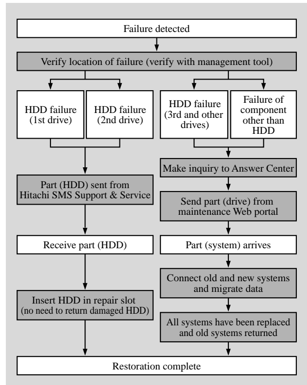
Fig. 6—Flow for Dealing with Array System Failures. Flow for dealing with system failures in maintenance operations is shown.
