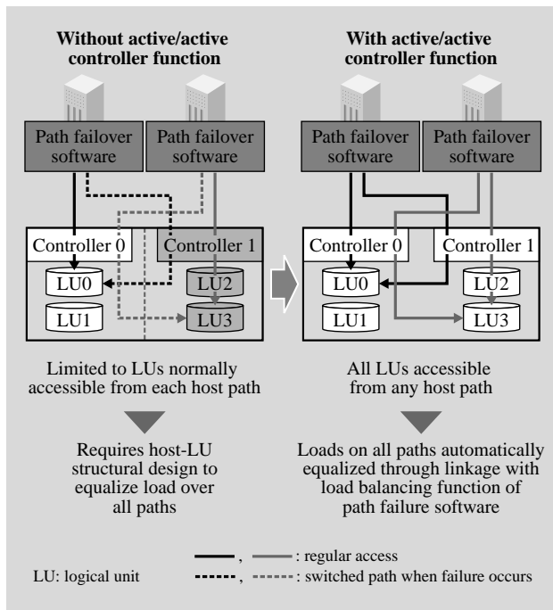
Fig. 3—Load Balancing Using the Active/active Controller. All LUs are accessible from any host path, and path efficiency has been optimized by the path failover software load balancing function.
