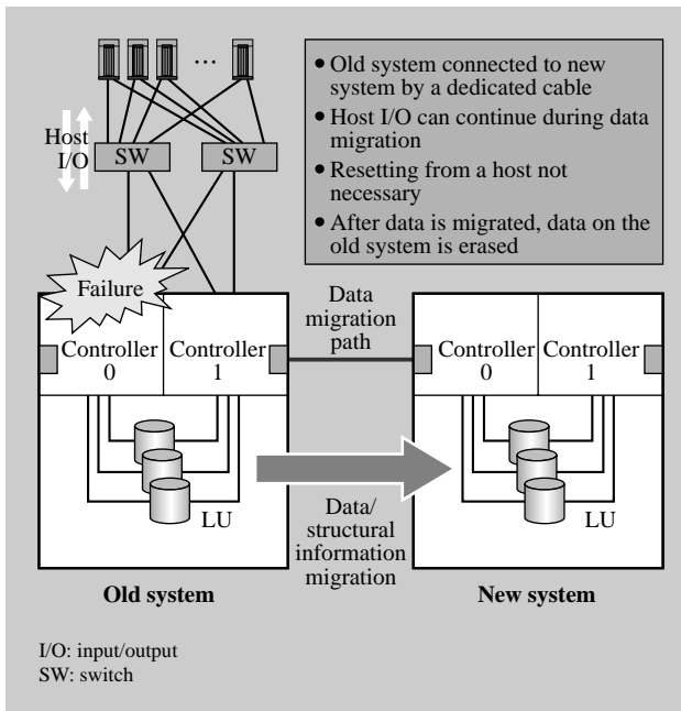
Fig. 5—Auto-migration of Data and Structural Information. Data is automatically migrated by following simple on-screen instructions, and work can continue on hosts connected to the disk array even while the data transfer is in progress.
