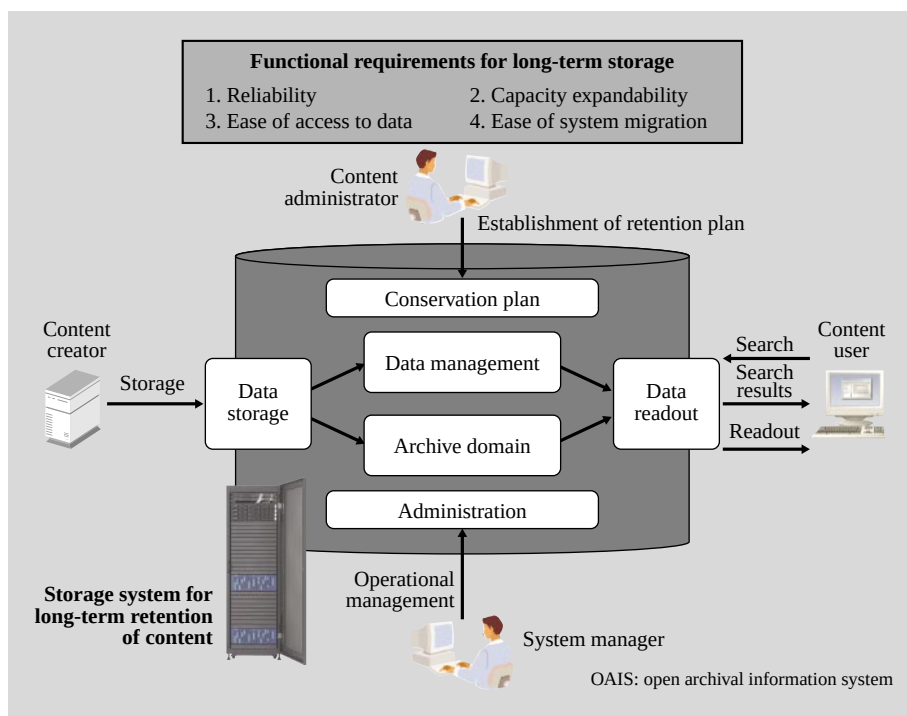
Fig. 2—Functional Requirements for Long-term Storage Based on OAIS Model.
