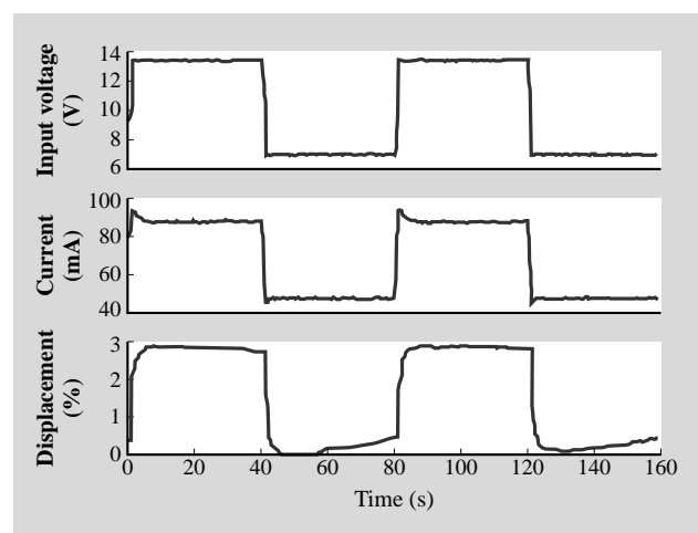
Fig. 7—Film Current and Displacement of the CNP Composite Actuator that Works in Air.
