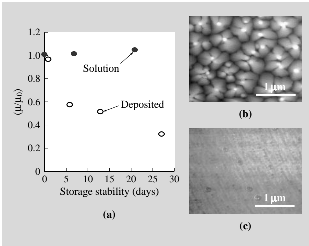
Fig. 4—Behavior of Pentacene for Different Processes. Comparison of storage stability for deposited versus solution-processed pentacene TFT (thin film transistor) (a), AFM (atomic force microscope) image of deposited pentacene surface (b), AFM image of solution-processed pentacene surface (c) are shown.
