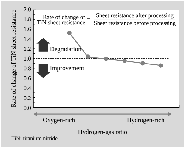
Fig. 4—Rate of Change of TiN Sheet Resistance with Increasing Hydrogen Ratio.
