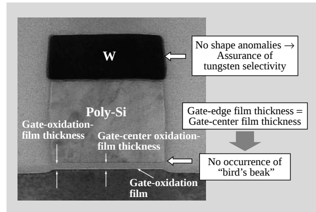
Fig. 5—Cross-sectional-TEM Assessment of Shape Formed by Selective-oxidation Processing.
