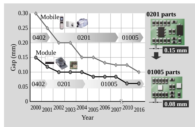
Fig. 3—Very Small Electrical Part Gap Requirements.
