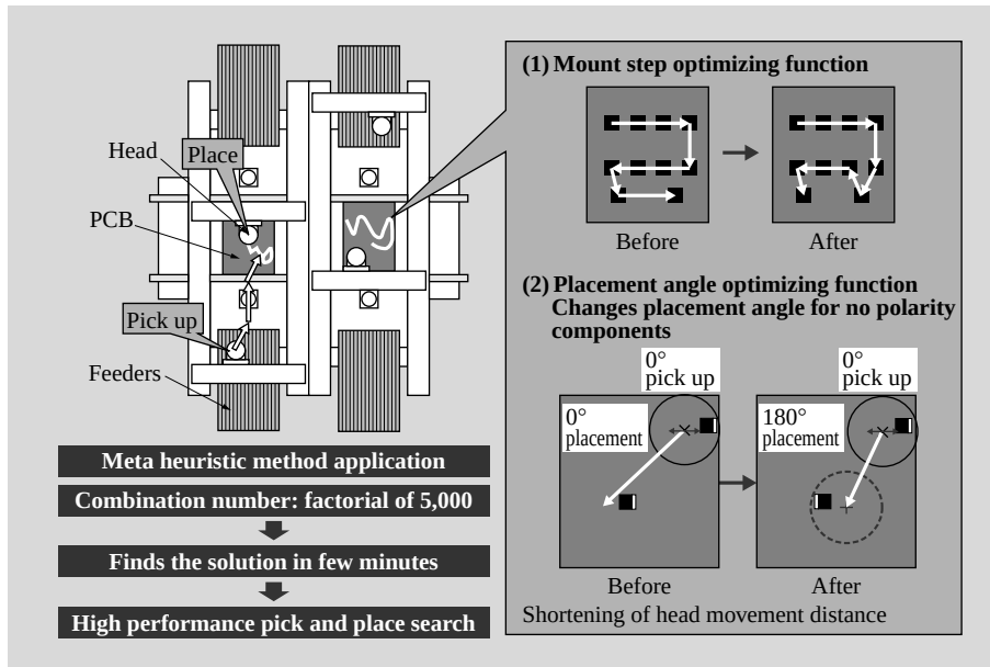
Fig. 13—Optimization Algorithm. Applying the meta heuristic method, optimum solutions are obtained in the least time and high performance pick and place sequence searches can be performed.
