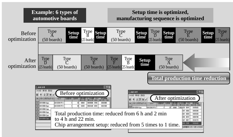
Fig. 14—Improved Productivity with the Multi-product Line Balance Software.
