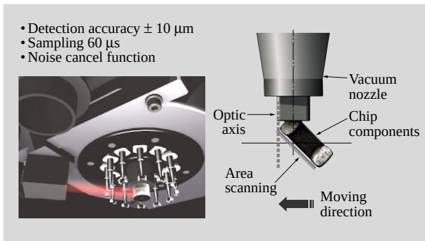
Fig. 11—Height to Bottom Surface of the Part Feedback. Checks the presence of components, inspects components, and discards defective parts. Also measures the height to the bottom surface of normal parts, and provides the information as feedback to determine the placement height.
