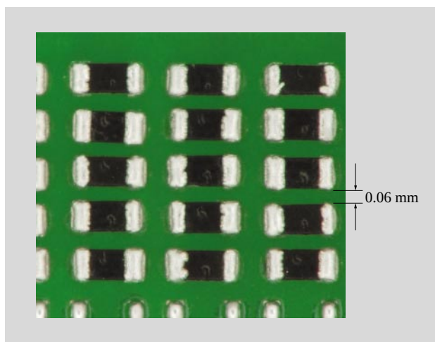
Fig. 15—Example of 01005R Placement after Reflow. The chip is placed with 0.06 mm gap in the Y direction.
