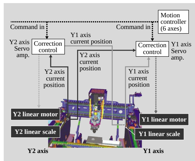
Fig. 7—Inter-axis Correction Control by Both-side Linear Motors. Respective positions of Y1 and Y2 axes are monitored and synchronized with each other.
