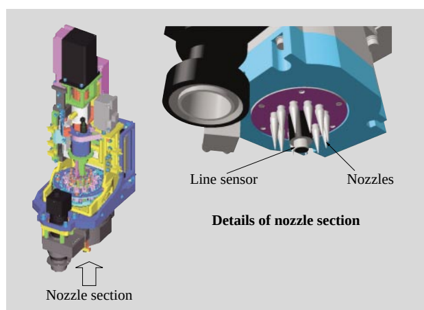
Fig. 5—Direct Drive Head.
