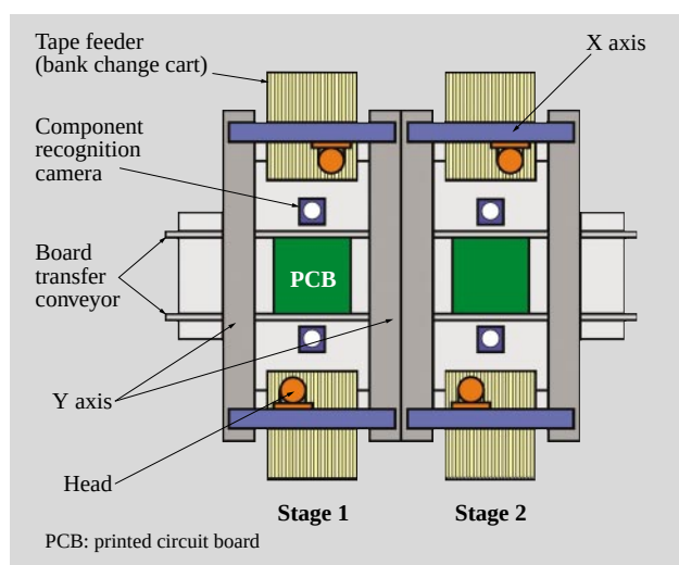
Fig. 4—GXH-3 Configuration. Equipped with two stages, four beams, and four heads, the GXH-3 mounts parts on two boards simultaneously.
