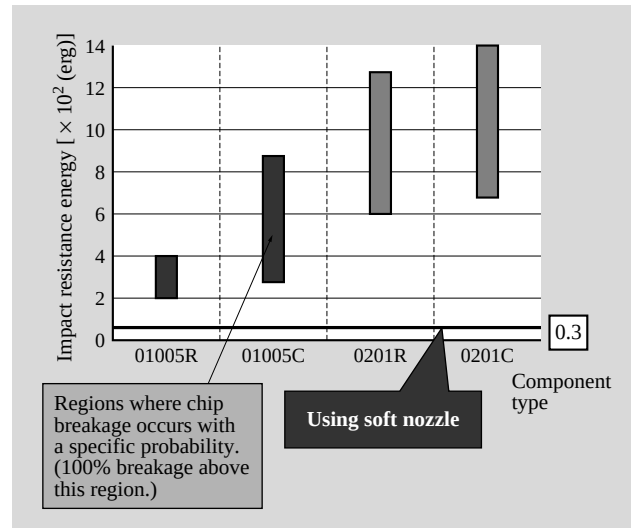
Fig. 12—Small Electrical Parts Brakeage Regions. Even for 01005R (0.4 mm \times 0.2 mm resistor) parts with the smallest impact resistance energy, the impact force is cushioned by the soft mounting nozzle.
