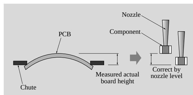
Fig. 10—Board Height Feedback.
