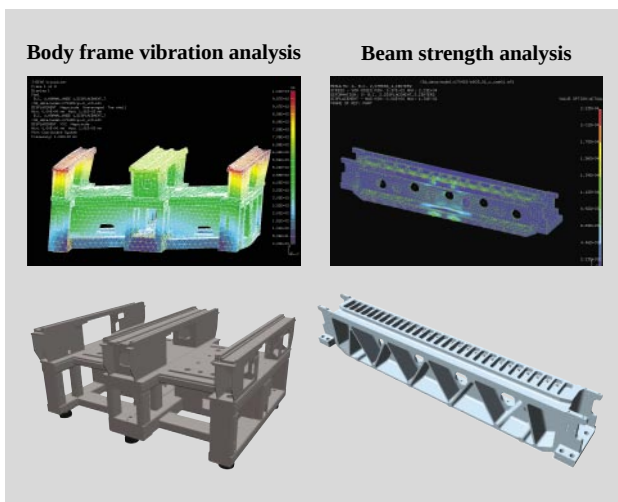
Fig. 6—Examples of CAE Analysis Results. Optimized design of characteristic values and strength is achieved through CAE (computer-aided engineering) analysis.
