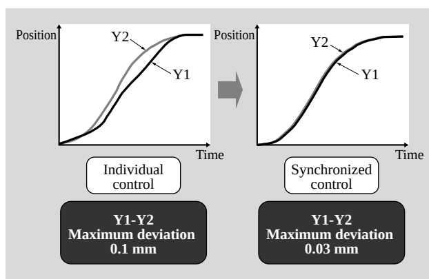
Fig. 8—Results Using Inter-axis Correction Control by Both-side Linear Motors.
