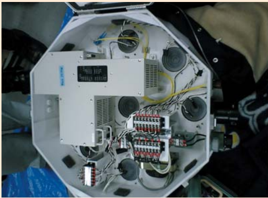
Small-scale control terminal (upper) and mounting (lower)
