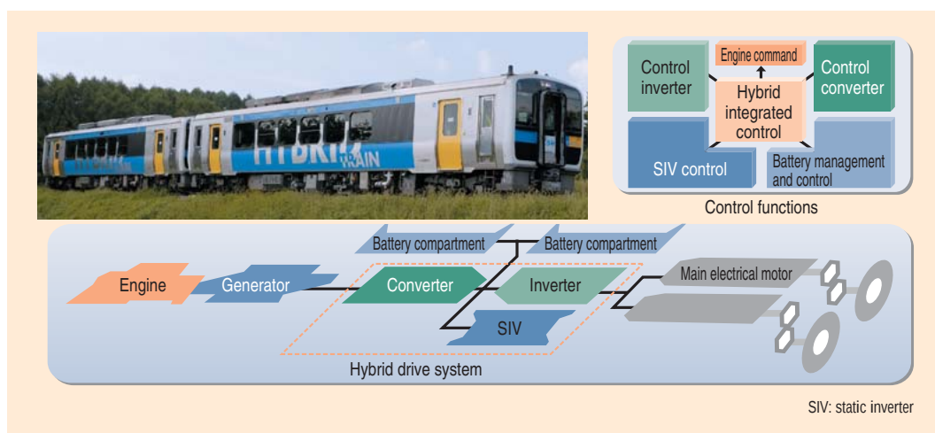
Exterior view of Kiha E200 car (upper left) and the structure of the hybrid drive system
