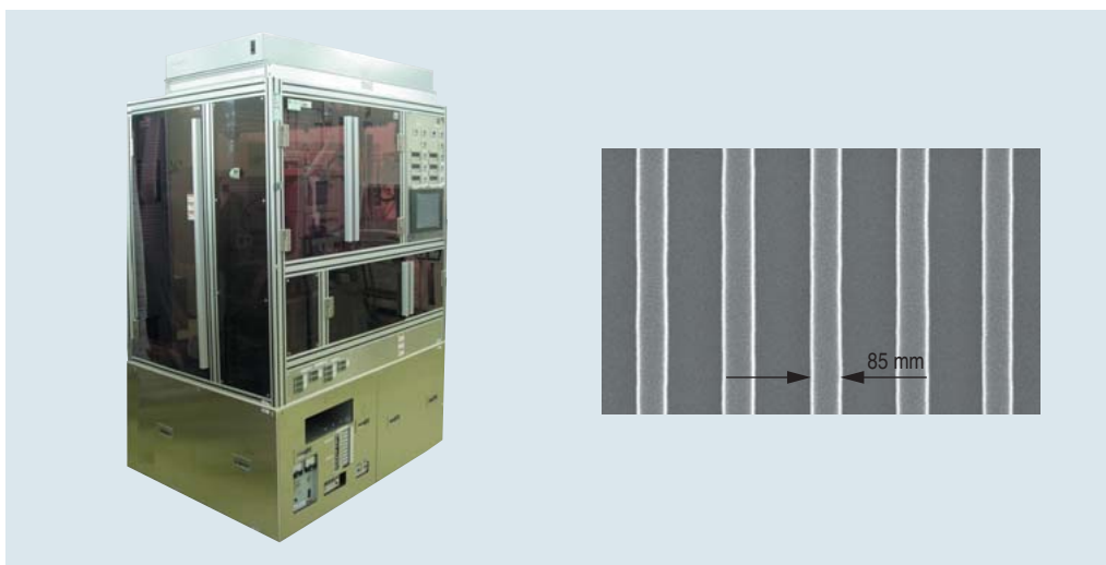
Photo-nanoimprint system (left) and the example of patterned polymer (right)
