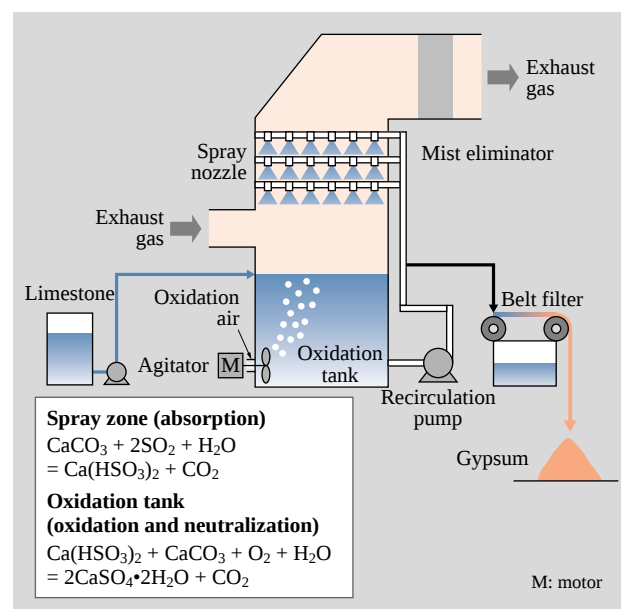
Fig. 5—Process Flow and Reaction Formulae for Desulphurization Equipment (In-situ Forced Oxidation System with Limestone-gypsum Process).
