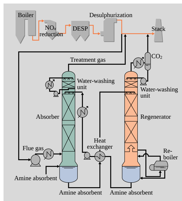
Fig. 7—Process Flow of \text{CO}_2 Recovery Pilot Plant ( 1,000 \text{ Nm}^3/\text{h} ). \text{CO}_2 in the flue gas is recovered by a newly developed amine solvent.
