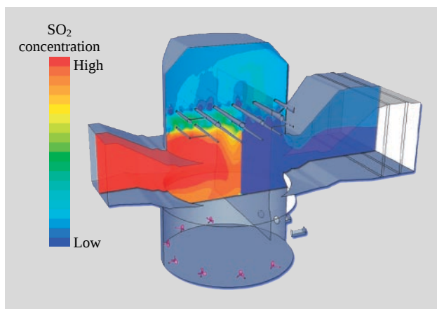
Fig. 6—Calculation Results on \text{SO}_2 Concentration in Desulphurization Unit. Distribution of \text{SO}_2 concentration in actual equipment is calculated accurately and contributes to compactification of the equipment.
