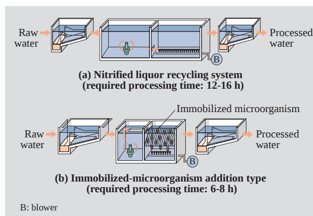
Fig. 4—Overview of Nitrogen-treatment System for Wastewater. By using entrapped immobilized microorganisms, it is possible to convert for nitrogen-removal processing without having to add reaction vessels of a conventional activated sludge process.
