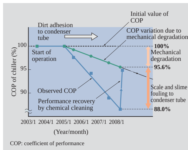
Fig. 4—Aging Degradation of Turbo Chiller (Diagnosing Result by Observation System).
