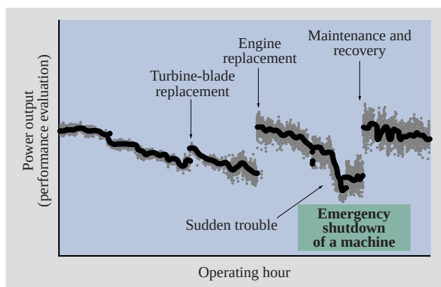
Fig. 3—Evaluation of a Gas Turbine Performance Degradation. Since aging deterioration of power output as well as performance restoration by maintenance and conditions for abrupt performance degradation can be quantified by use of developed software, appropriate maintenance can be carried out. And trouble due to sudden performance degradation can be forecasted.
