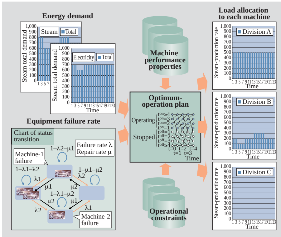
Fig. 5—Planning System for Optimum Design.
