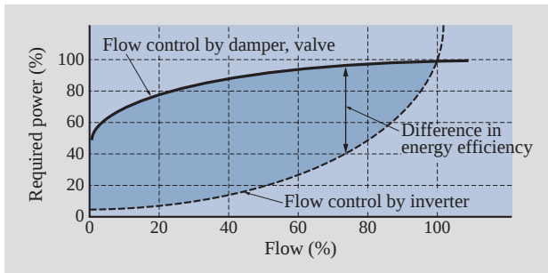
Fig. 2—Relation Between Flow and Required Power.
