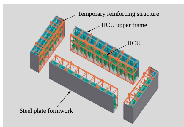
Fig. 3—Structure of Conventional HCU Module.
