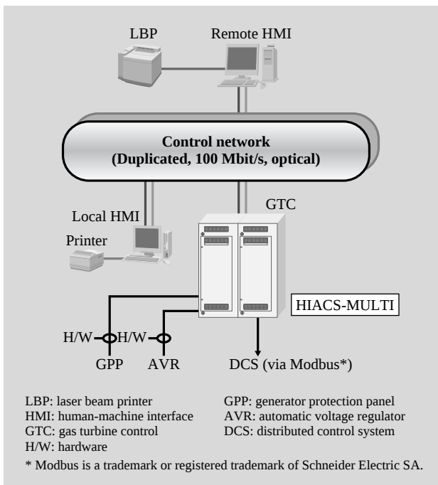
Fig. 3—System Configuration.
