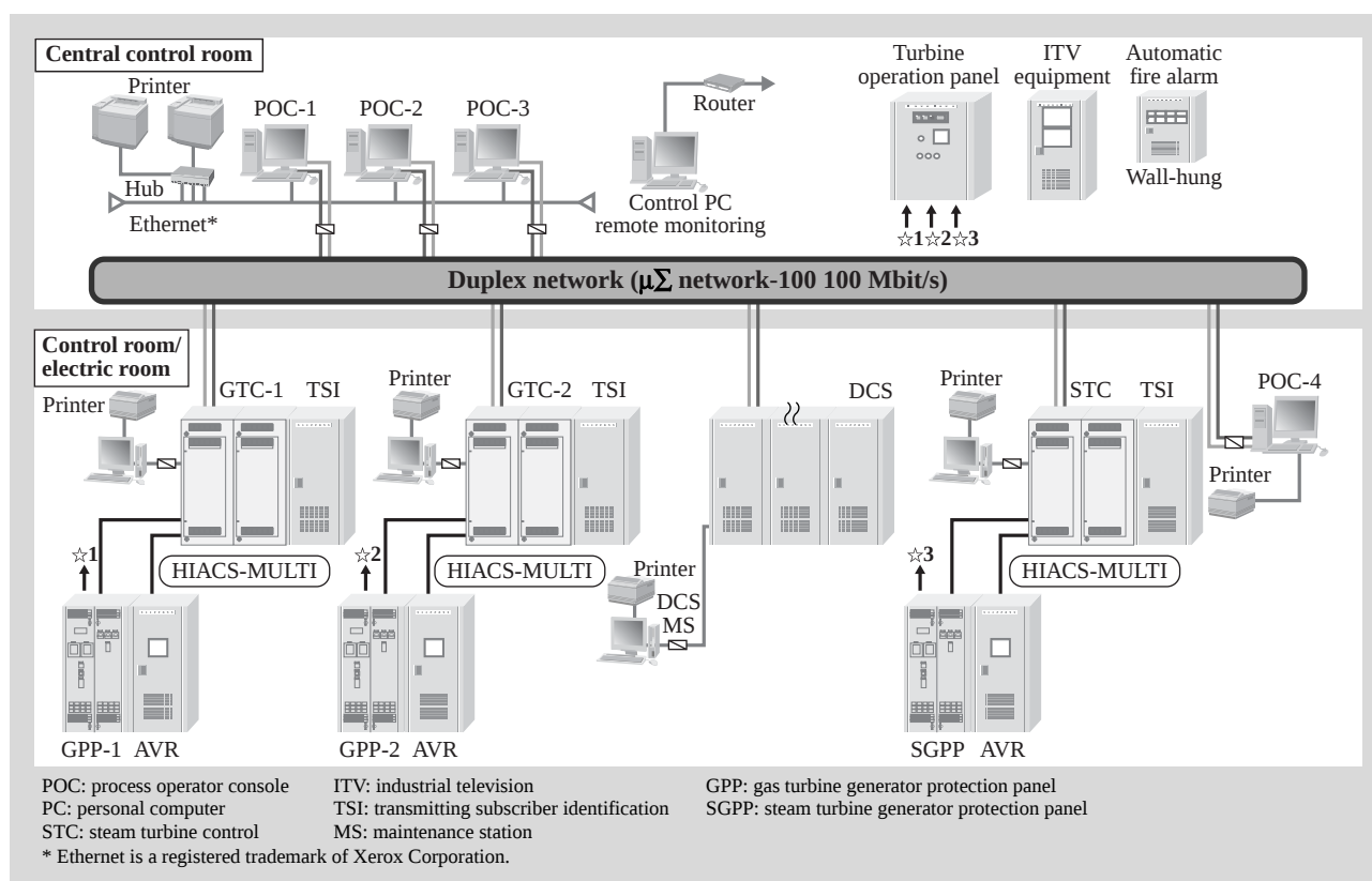
Fig. 6—Typical HIACS-MULTI Deployment.
