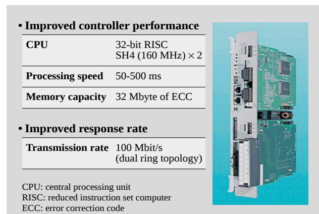
Fig. 4—Photo and Specifications of Hitachi CPU LPU610A.
