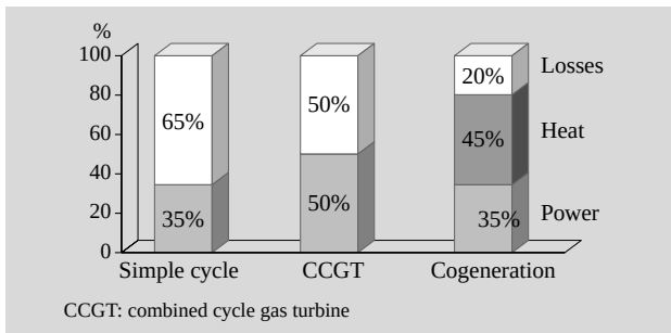
Fig. 4—Energy Efficiency Improvements.
