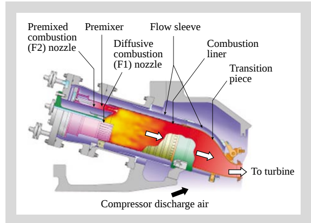
Fig. 3—LNC Cross Section.
