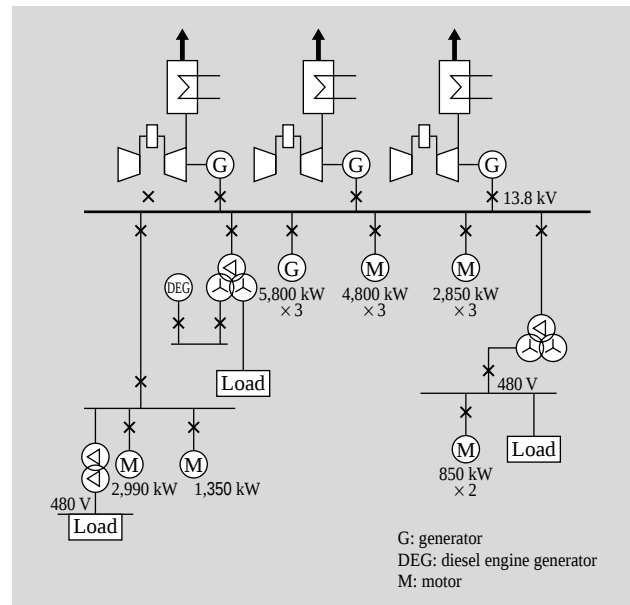
Fig. 8—Electrical System of Betara H-25 Plant. Three H-25 gas turbines are connected to 13.8 kV line and supply electricity to the motors for gas compressors.
