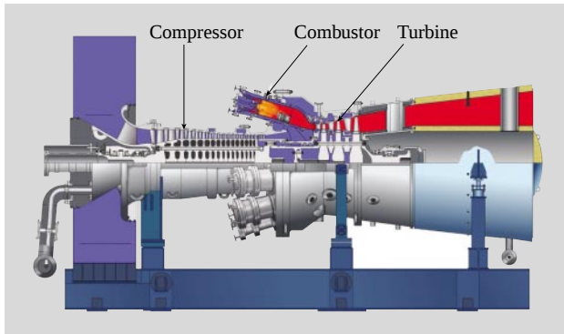
Fig. 2—H-25 Cross Section.
