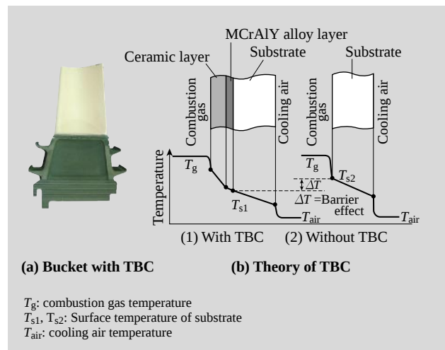
Fig. 4—TBC Technology for H-25 Gas Turbines.
