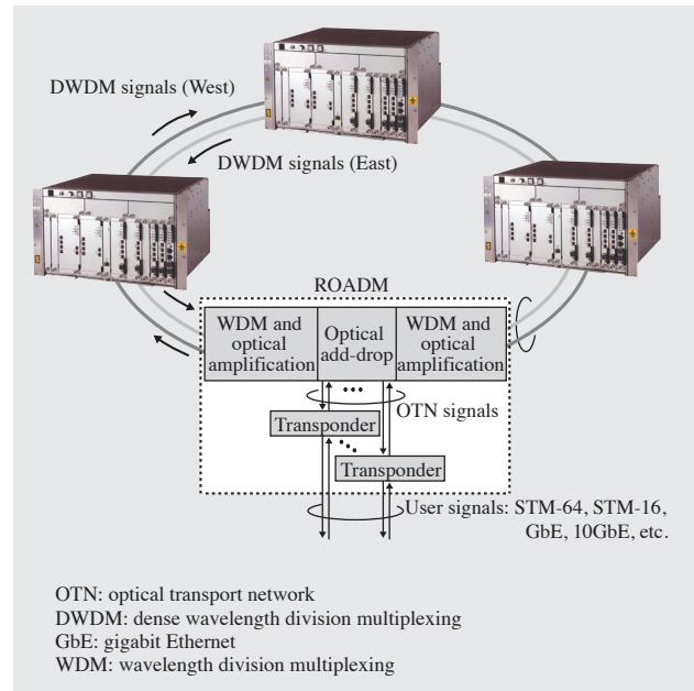
Fig.3—ROADM.
