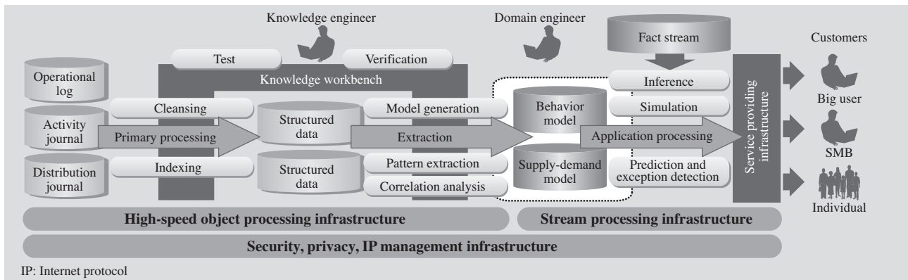
Fig. 6—Architecture of Knowledge Extracting Infrastructure.
