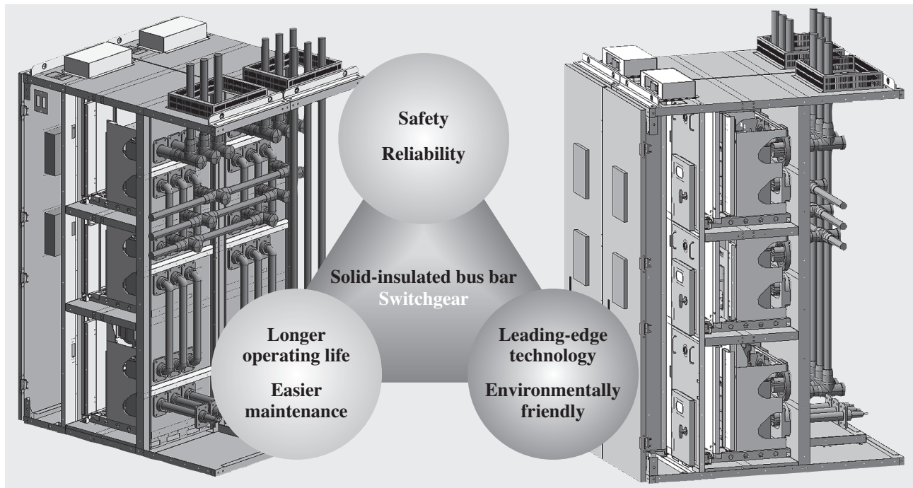
Fig. 1—Concepts Behind Switchgear with Solid-insulated Bus Bars.
