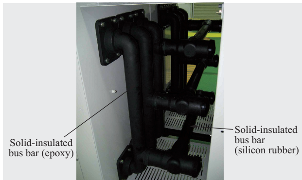
Fig. 3—View of Solid-insulated Bus Bars.
