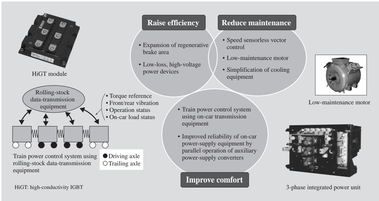
Fig. 4— Train Traction Solution. Hitachi proposes a train traction system that covers the need for high efficiency, easier maintenance, and improved passenger comfort.
