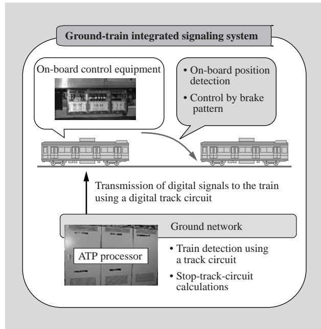
Fig. 9— Configuration of Digital ATP System. Hitachi proposes a digital ATP system that aims to achieve high-density service for easing congestion in high-density railway sections, decrease ground facilities, and improve maintainability.
