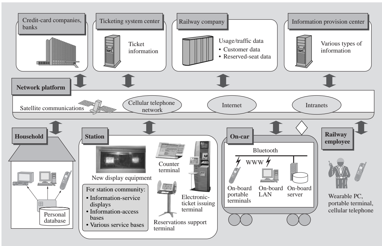
Fig. 10— Concept of Information Service Systems for Railways. Hitachi proposes information-service-system solutions to enhance railway-user services and support expansion of railway companies into the information services field.
