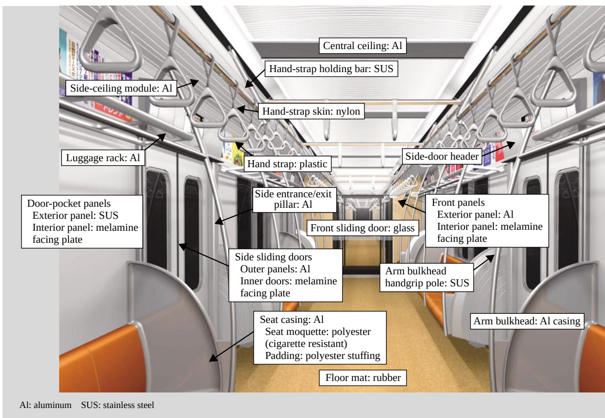
Fig. 7—Countermeasures against Fire and Noxious Gases for Passenger-cabin Fixtures. Materials for suppressing generation of fire and noxious gas are adopted for all fixtures (from the ceiling to seating and flooring materials).
