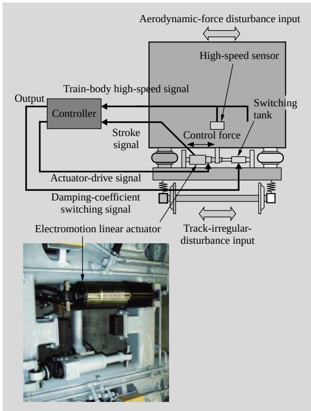
Fig. 4—Control Equipment for Preventing Shaking by Electromotion Linear Actuator.
