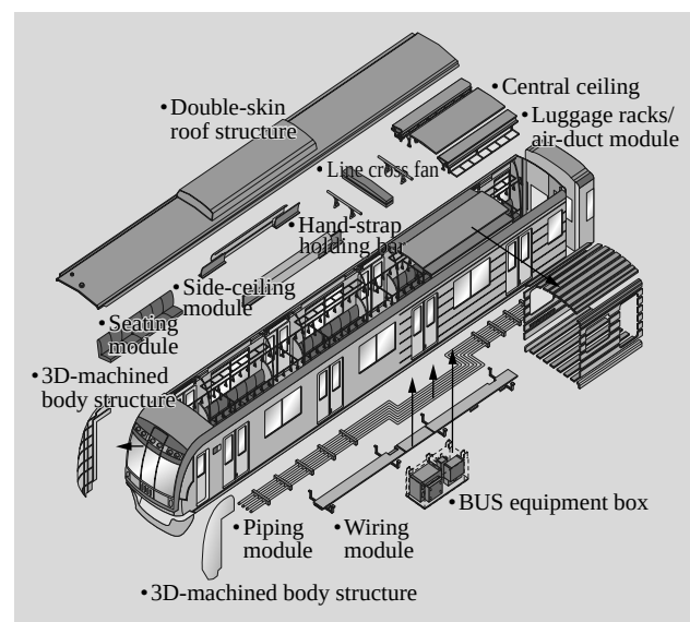
Fig. 5—Basic Structure of “A-train.”
