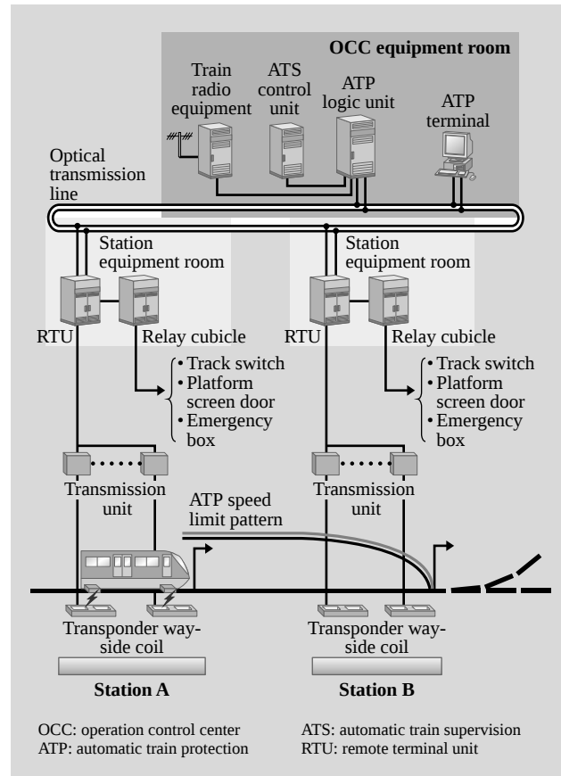
Fig. 3—Signaling System Schematic.
