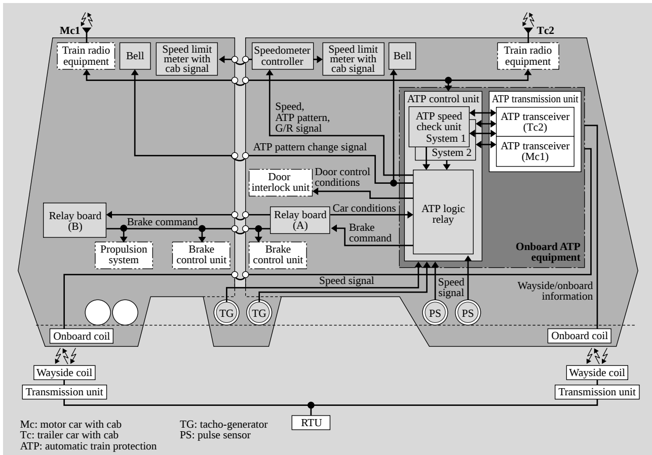
Fig. 4—Onboard ATP System Schematic.
