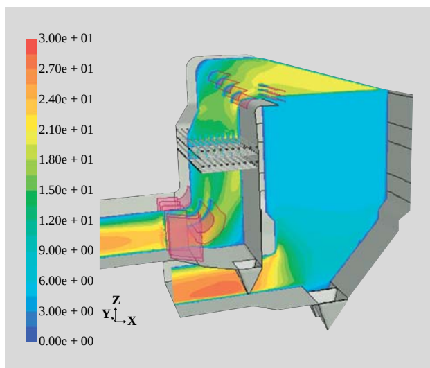
Fig. 3—Distribution of Flue Gas Flow in SCR Reactor Simulated by CFD (computational fluid dynamics). Based on the CFD results, the flow model test was also conducted to verify the final results.
