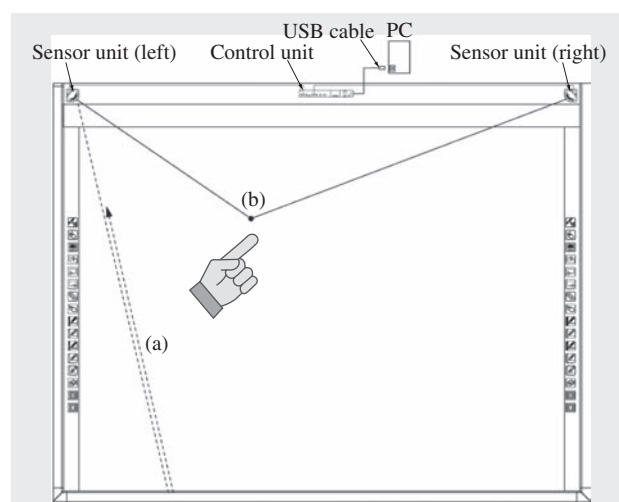
Fig. 6—StarBoard FX-DUO Operating Principles.
