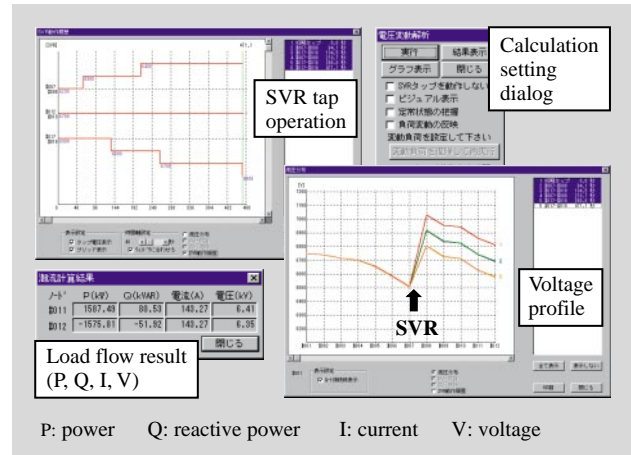
Fig. 2—Example Results of Voltage Fluctuation Simulations. Trends in SVR tap operation, line power flow, and profile of node voltage are indicated both by numeric values and charts.
