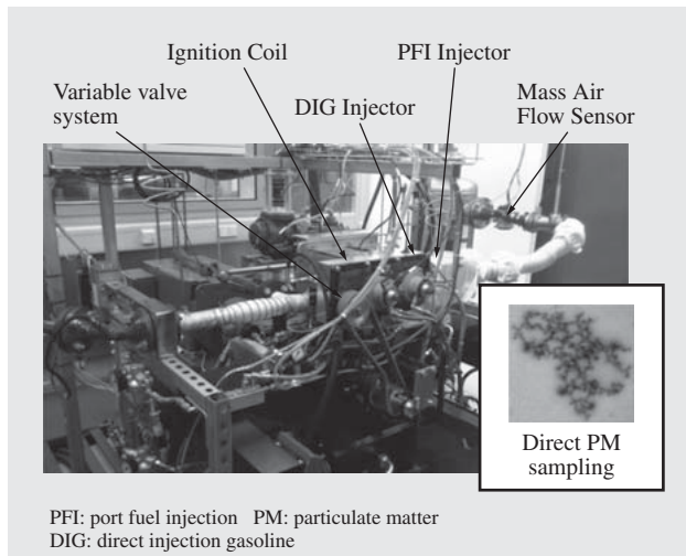
Fig. 1—Single-cylinder Research Engine at TUM. The engine includes Hitachi components and is used to conduct combustion analysis and emission measurements for simulation model development.
