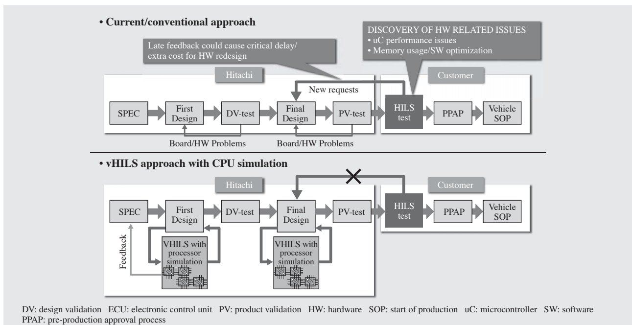
Fig. 6—Benefits of vHILS and its Role in Controller Development Cycle.
