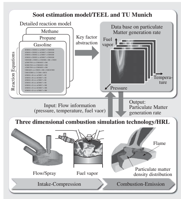
Fig. 2—Three-dimensional Combustion Technology for Analyzing Mechanisms of Particulate Matter Generation. TEEL and TUM have developed a detailed reaction model and a framework that links the detailed chemical model and three-dimensional combustion simulation technology.
