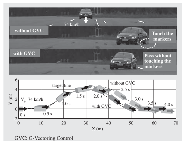
Fig. 4—Result of evaluation test in Germany. Double lane change test called “elk test” was performed as the evaluation test of GVC. GVC could improve the obstacle avoidance performance without discomfort.
