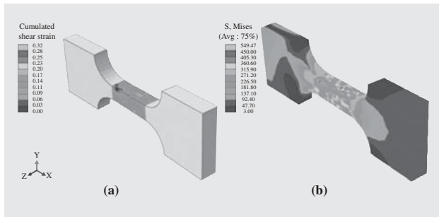
Fig. 9—CPFEM Model for Simulating Uniaxial Tensile Testing. The SUS316 material is assumed to have a random crystalline orientation. The results show: (a) cumulative shear strain over all slip systems in the gage section, and (b) Mises stress over the whole specimen.
